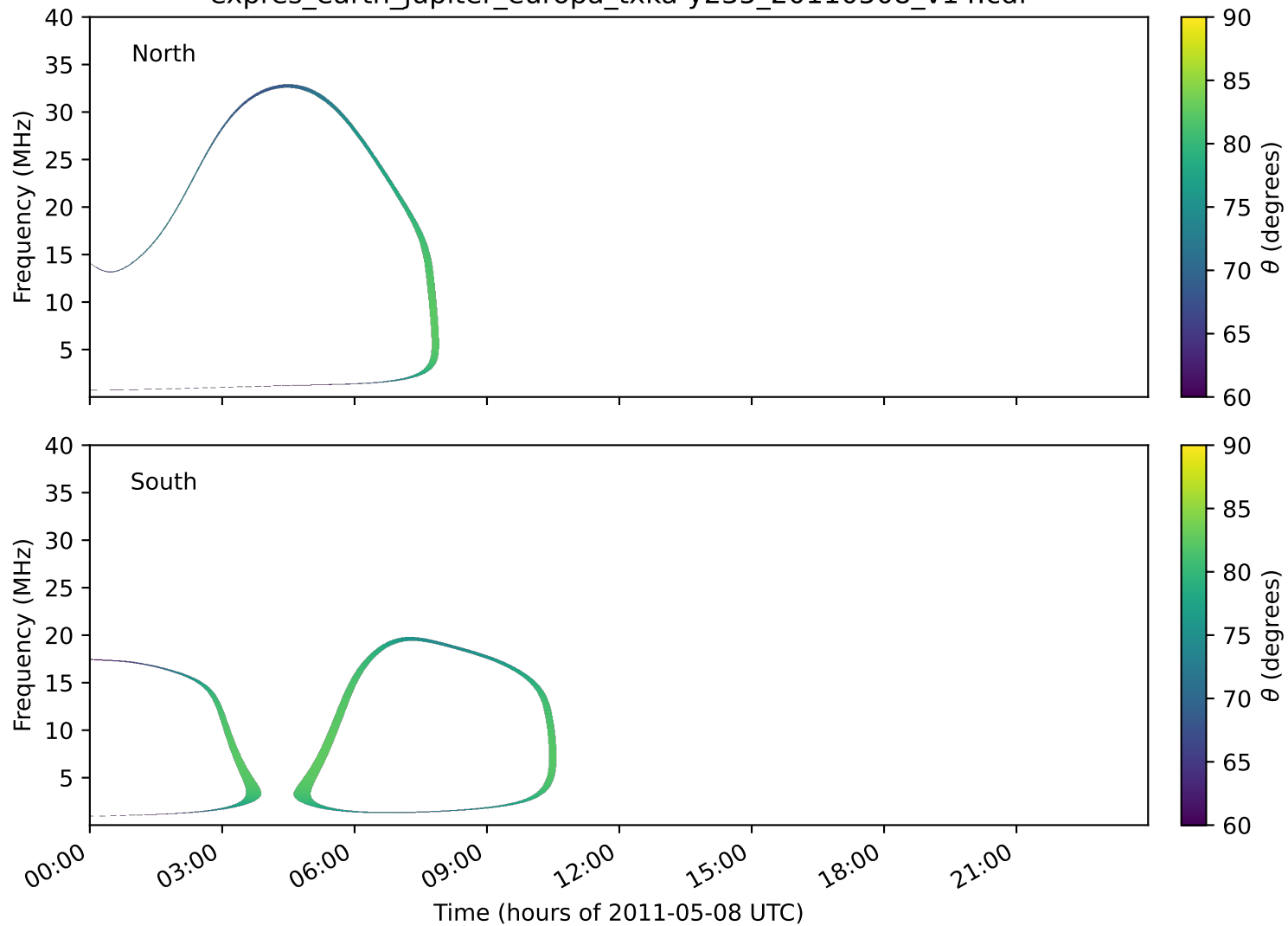
expres_earth_jupiter_europa_txka-y235_20110508_v14.cdf
