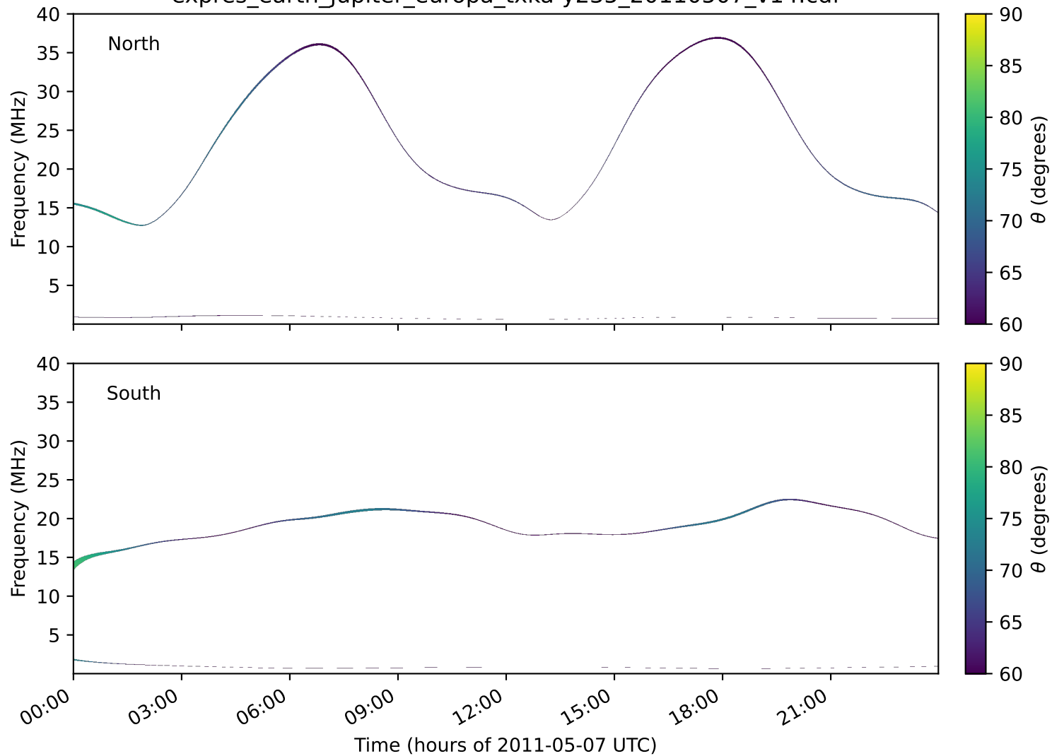
expres_earth_jupiter_europa_txka-y235_20110507_v14.cdf
