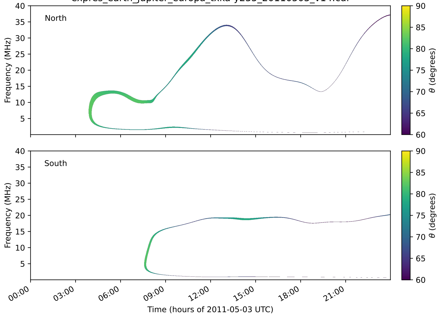
expres_earth_jupiter_europa_txka-y235_20110503_v14.cdf
