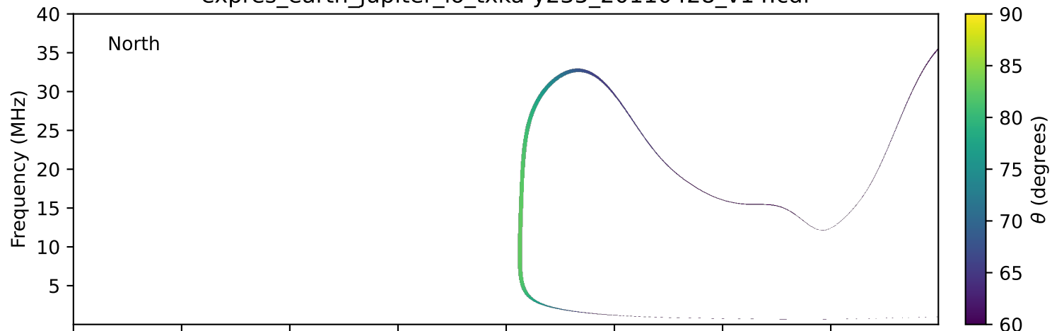
expres_earth_jupiter_io_txka-y235_20110428_v14.cdf
