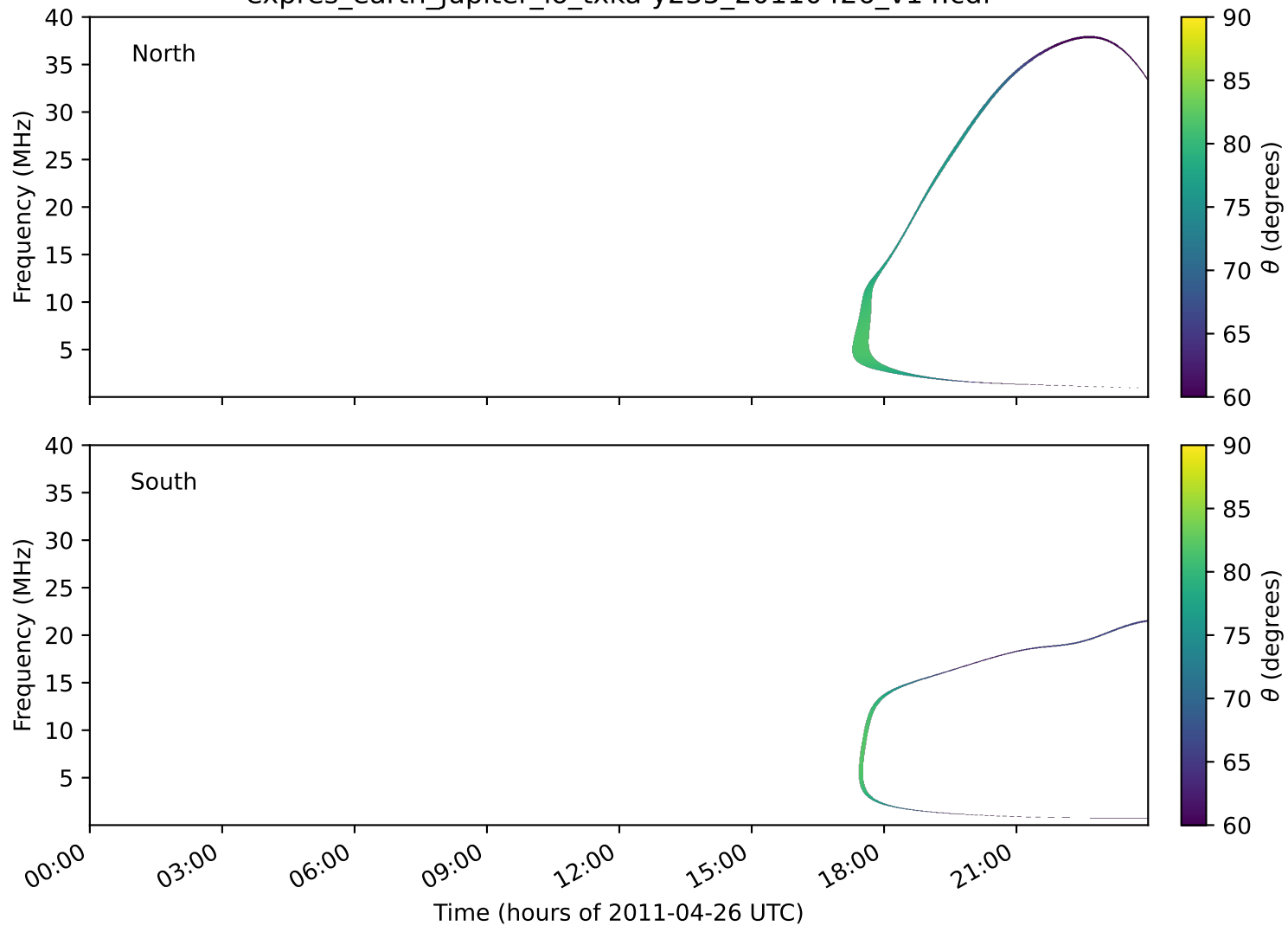
expres_earth_jupiter_io_txka-y235_20110426_v14.cdf
