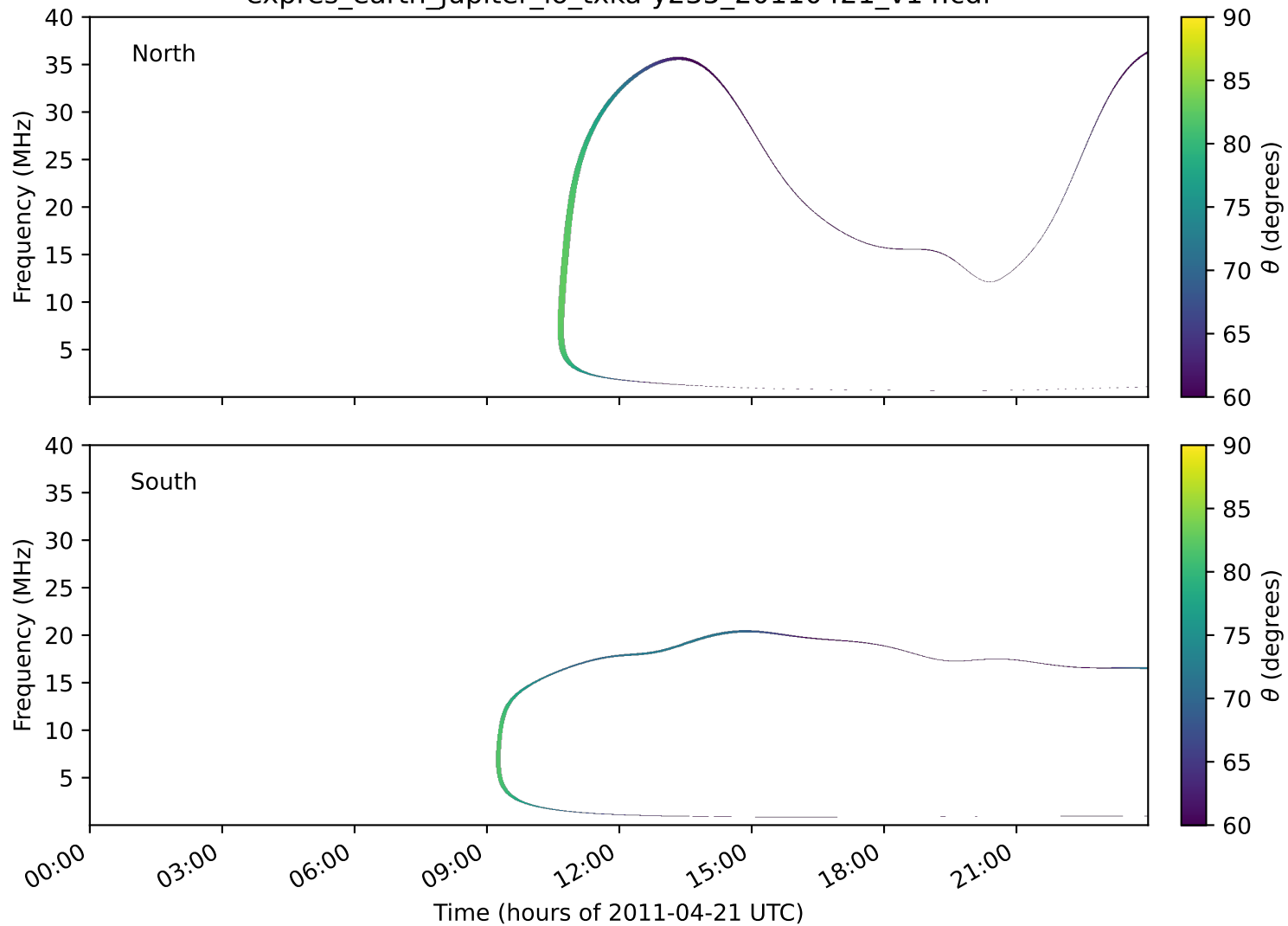
expres_earth_jupiter_io_txka-y235_20110421_v14.cdf
