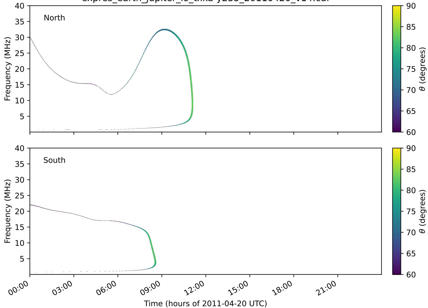
expres_earth_jupiter_io_txka-y235_20110420_v14.cdf
