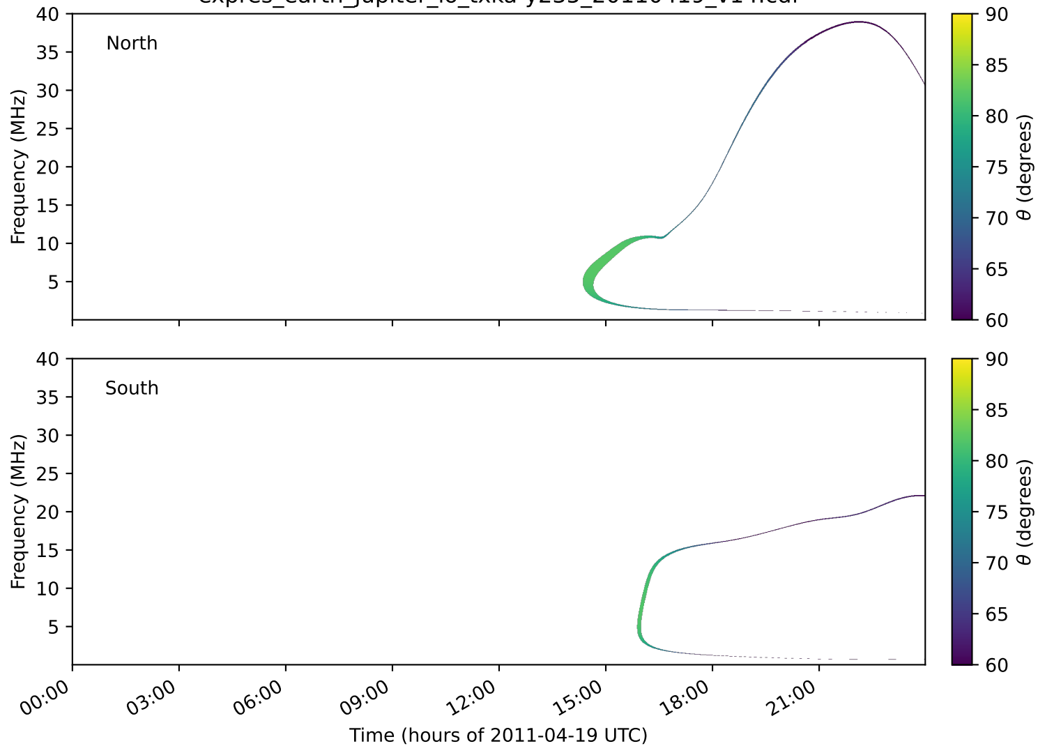
expres_earth_jupiter_io_txka-y235_20110419_v14.cdf
