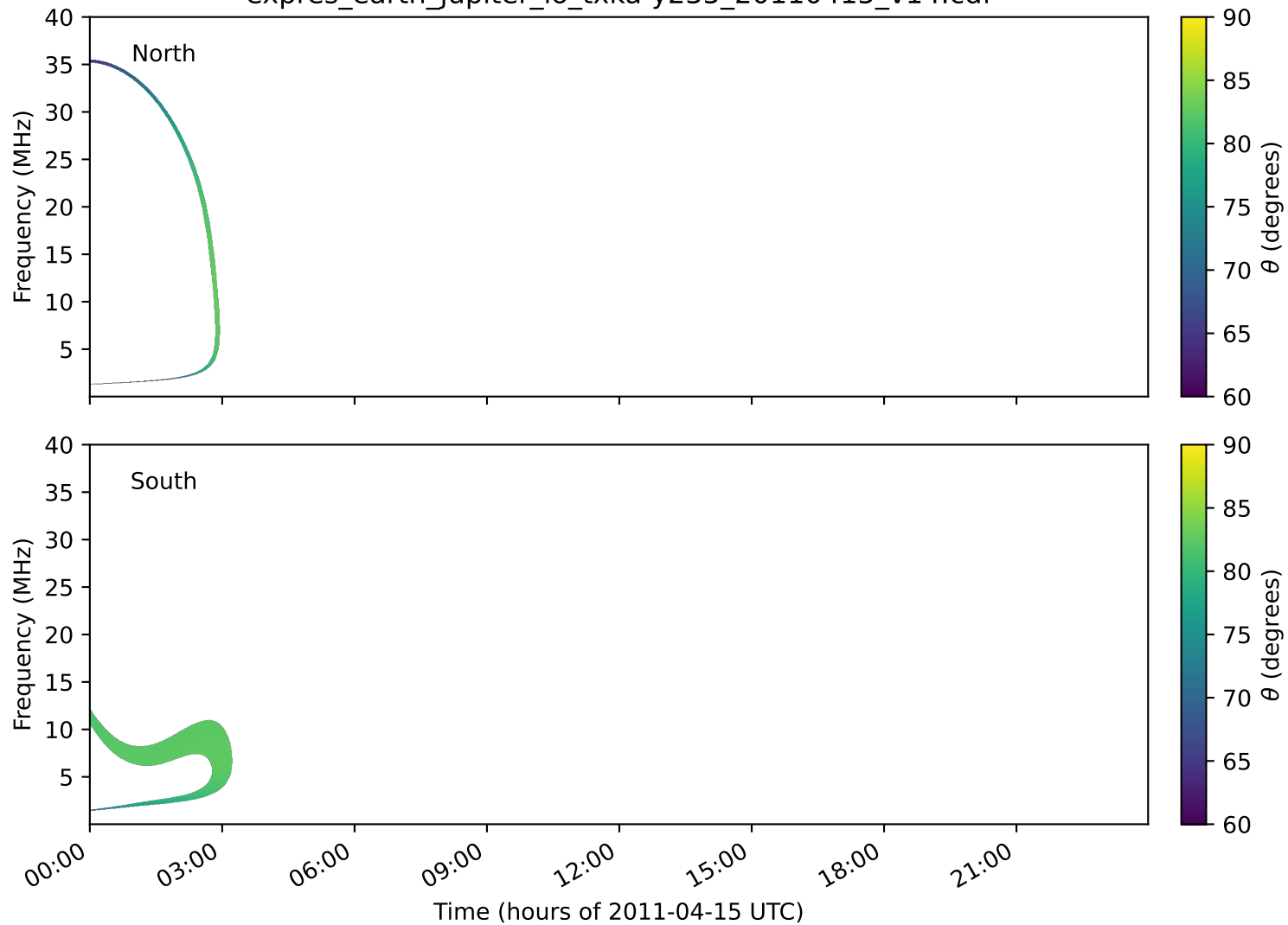
expres_earth_jupiter_io_txka-y235_20110415_v14.cdf
