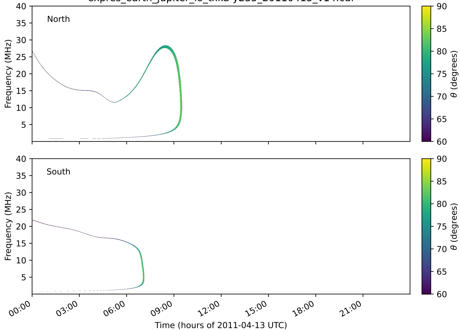
expres_earth_jupiter_io_txka-y235_20110413_v14.cdf
