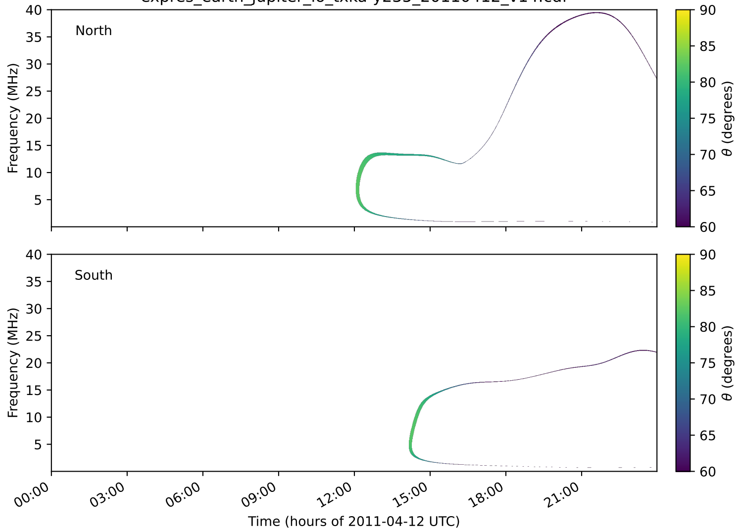
expres_earth_jupiter_io_txka-y235_20110412_v14.cdf
