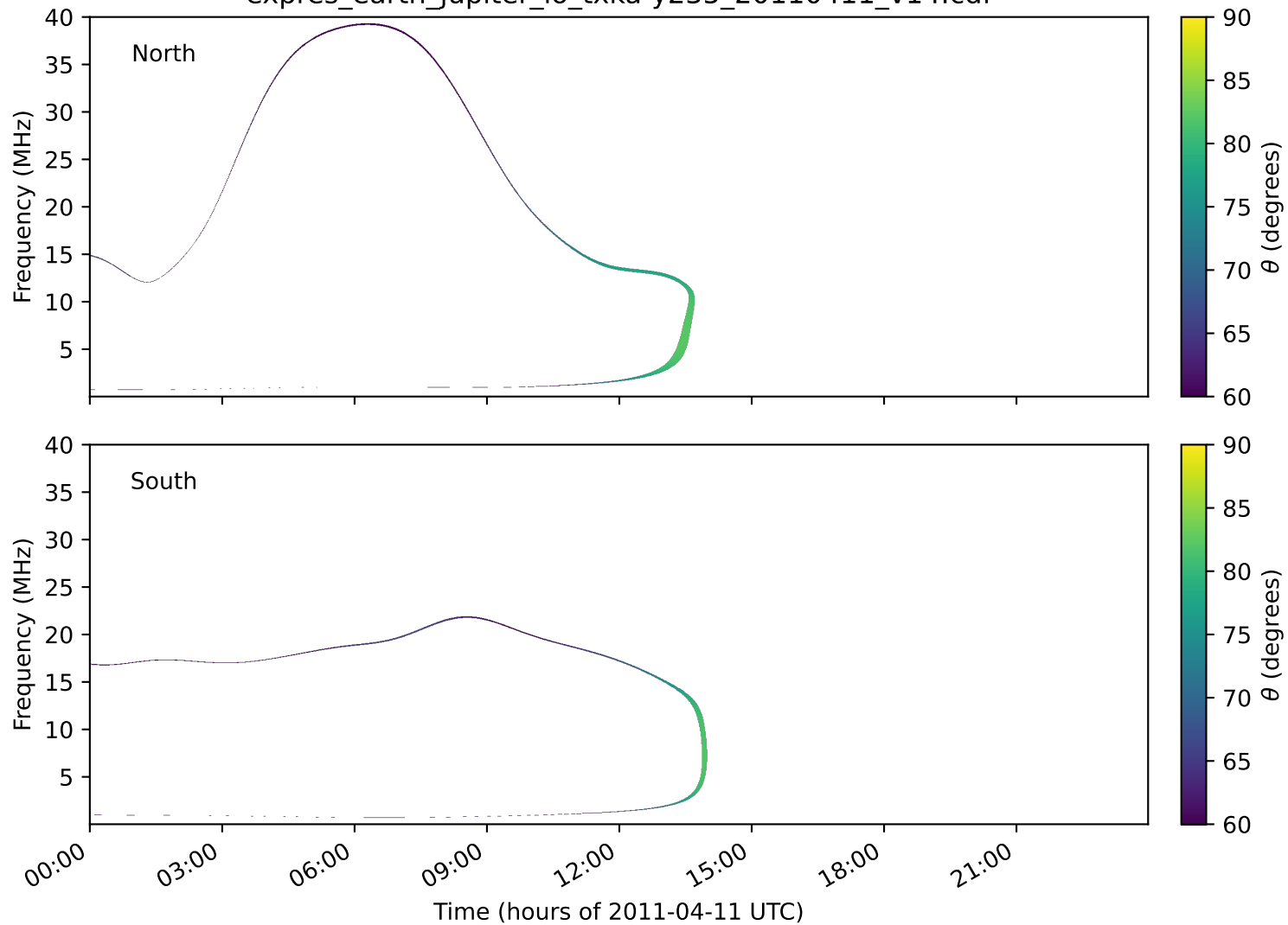
expres_earth_jupiter_io_txka-y235_20110411_v14.cdf
