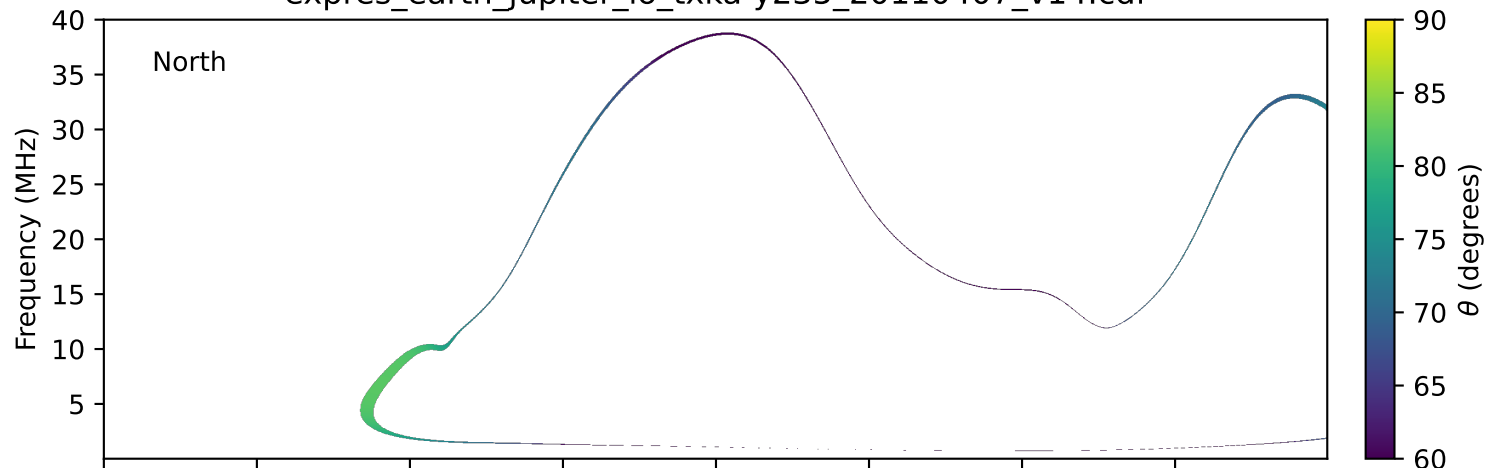
expres_earth_jupiter_io_txka-y235_20110407_v14.cdf
