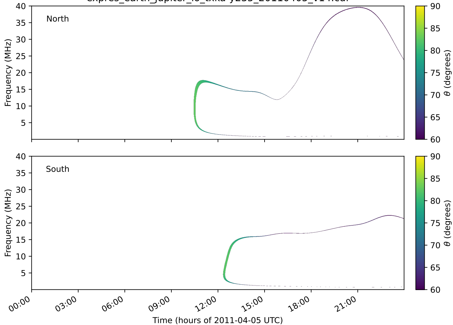
expres_earth_jupiter_io_txka-y235_20110405_v14.cdf
