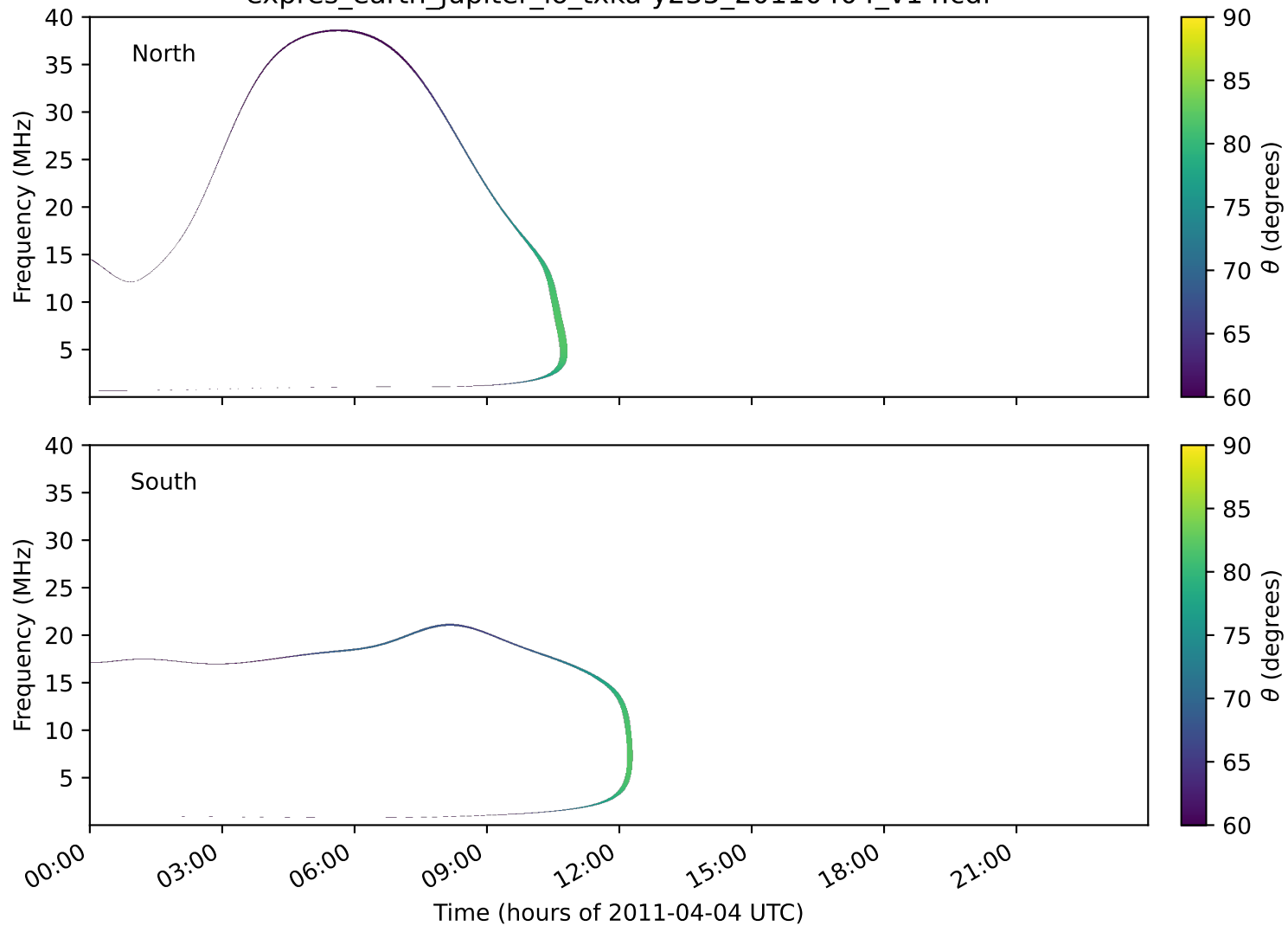
expres_earth_jupiter_io_txka-y235_20110404_v14.cdf
