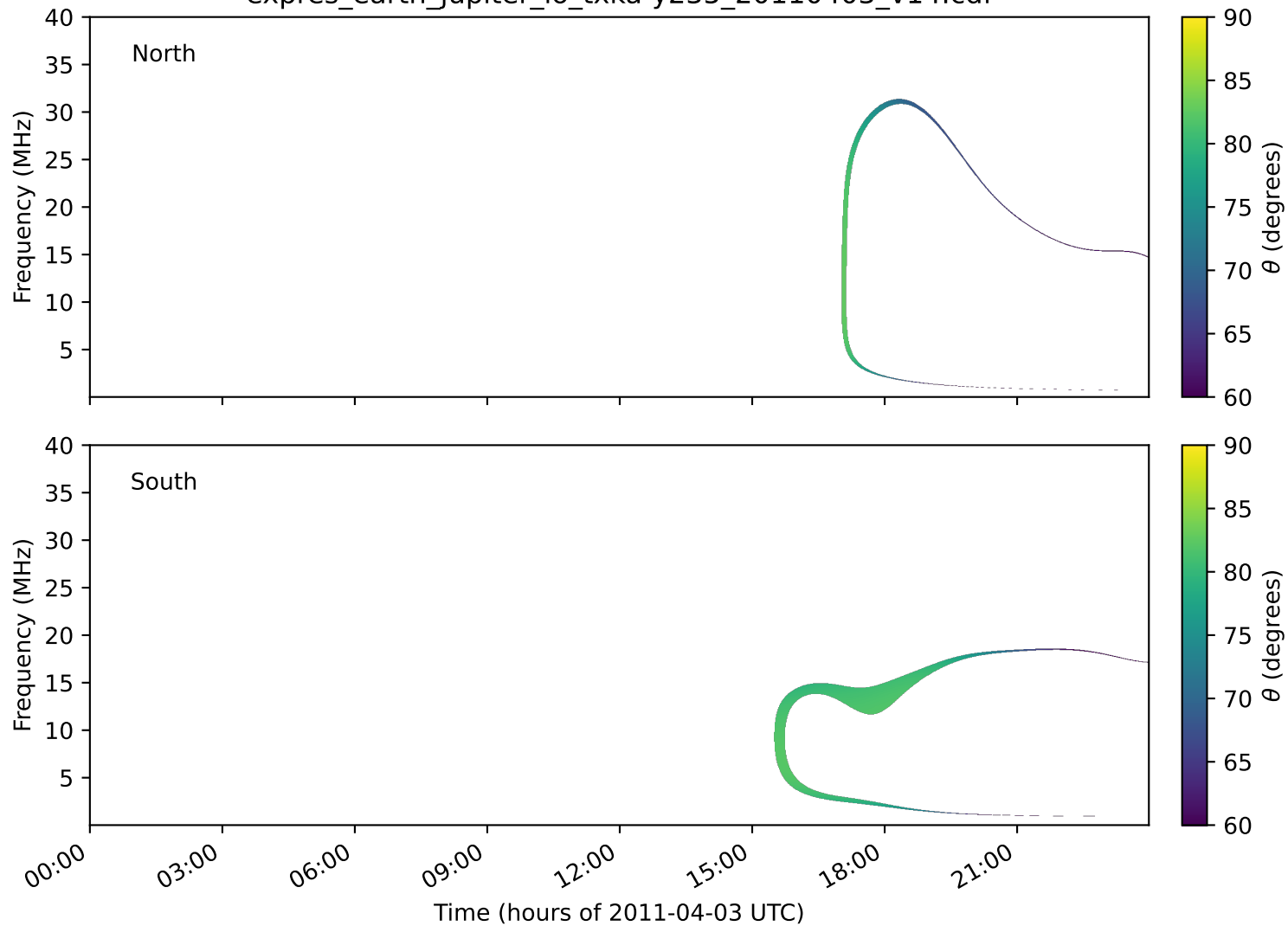
expres_earth_jupiter_io_txka-y235_20110403_v14.cdf
