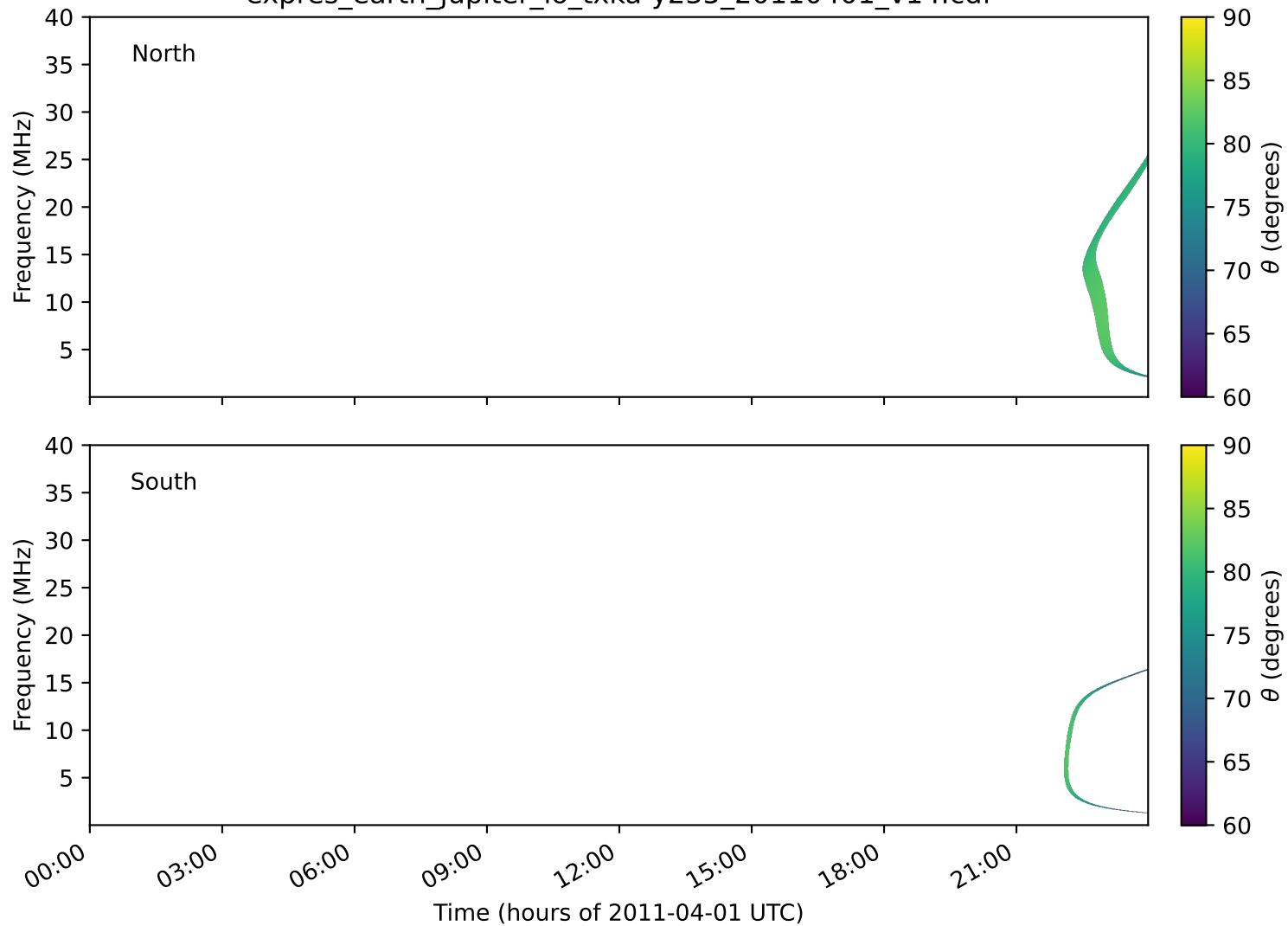
expres_earth_jupiter_io_txka-y235_20110401_v14.cdf
