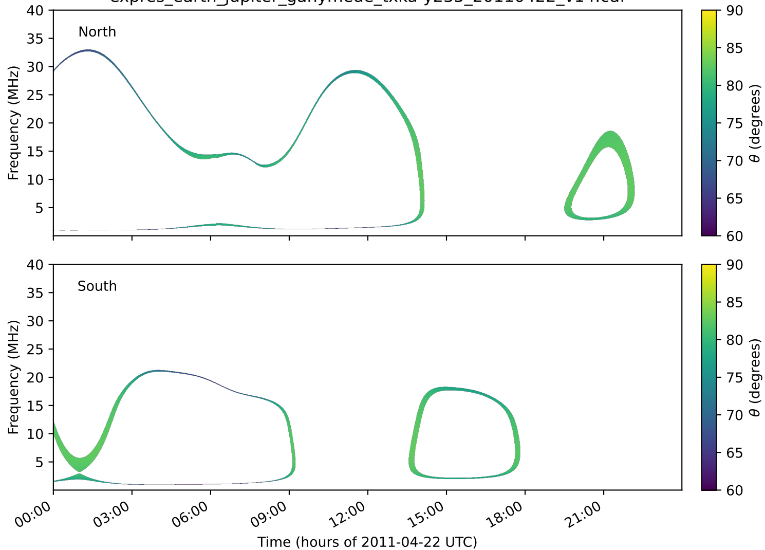
expres_earth_jupiter_ganymede_txka-y235_20110422_v14.cdf
