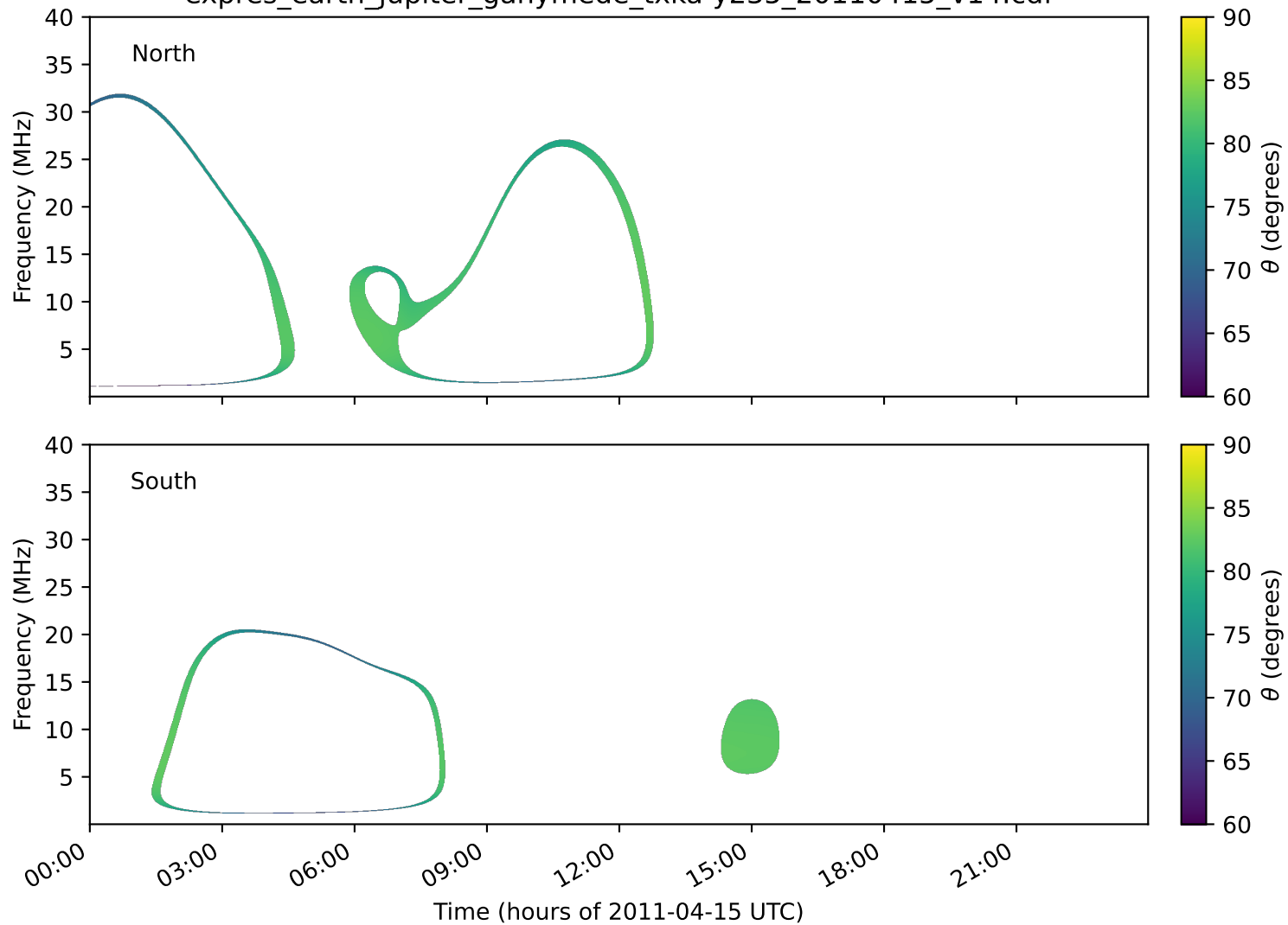
expres_earth_jupiter_ganymede_txka-y235_20110415_v14.cdf
