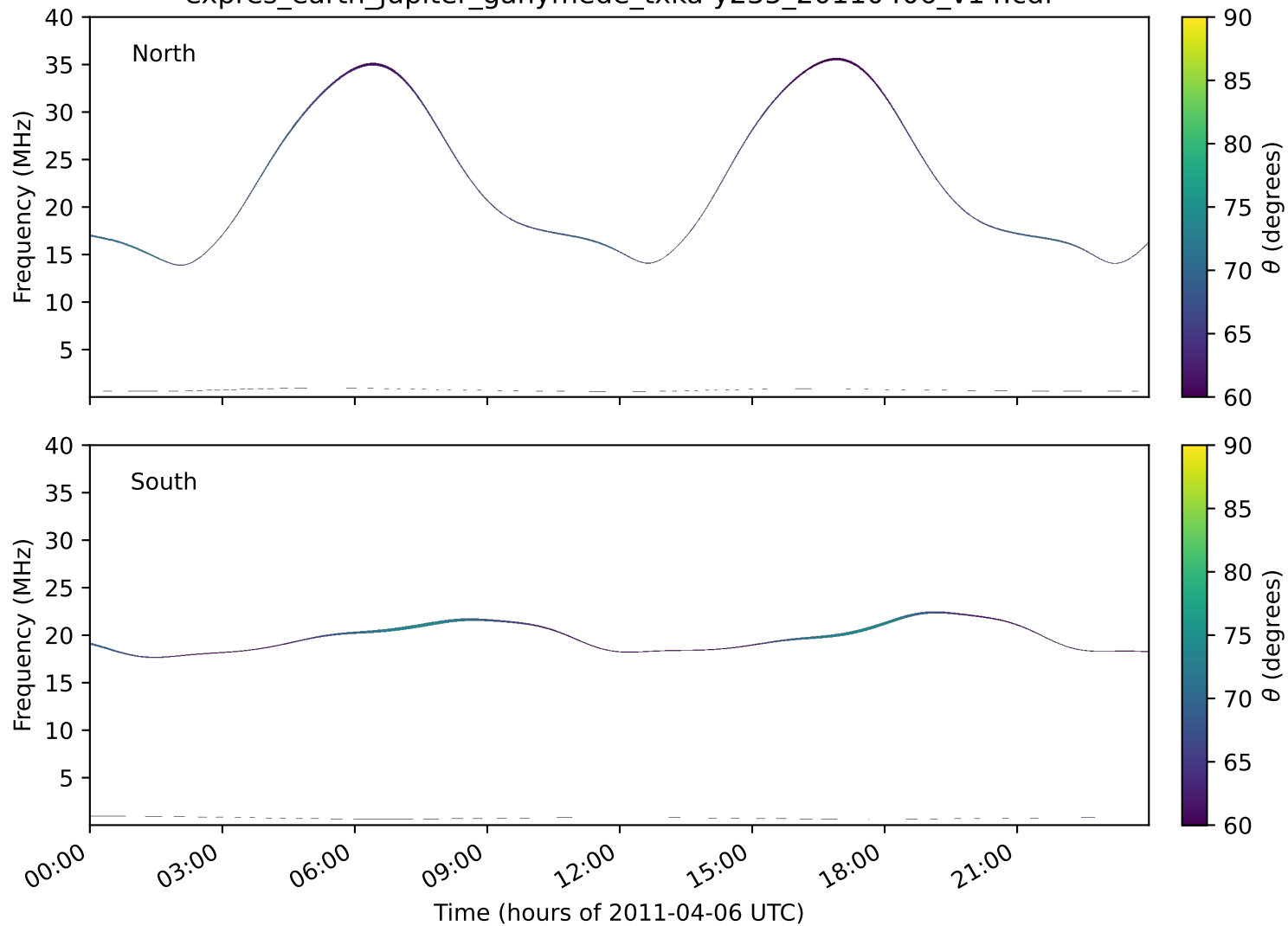
expres_earth_jupiter_ganymede_txka-y235_20110406_v14.cdf
