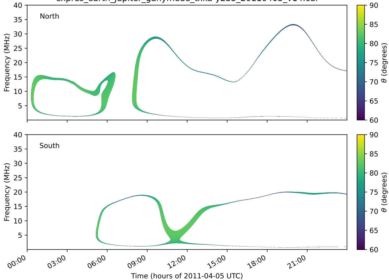
expres_earth_jupiter_ganymede_txka-y235_20110405_v14.cdf
