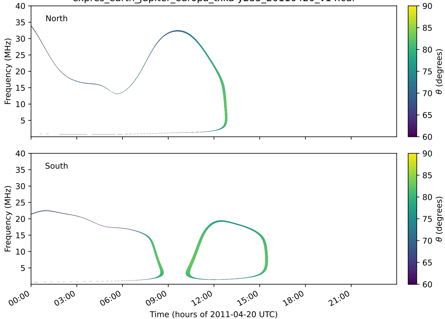
expres_earth_jupiter_europa_txka-y235_20110420_v14.cdf
