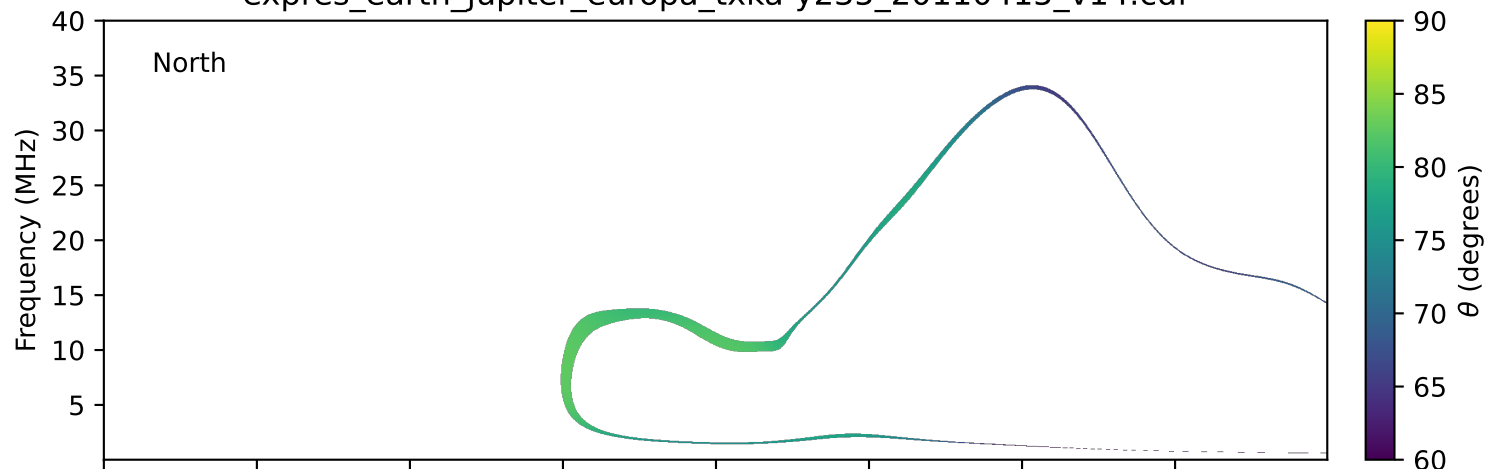
expres_earth_jupiter_europa_txka-y235_20110415_v14.cdf
