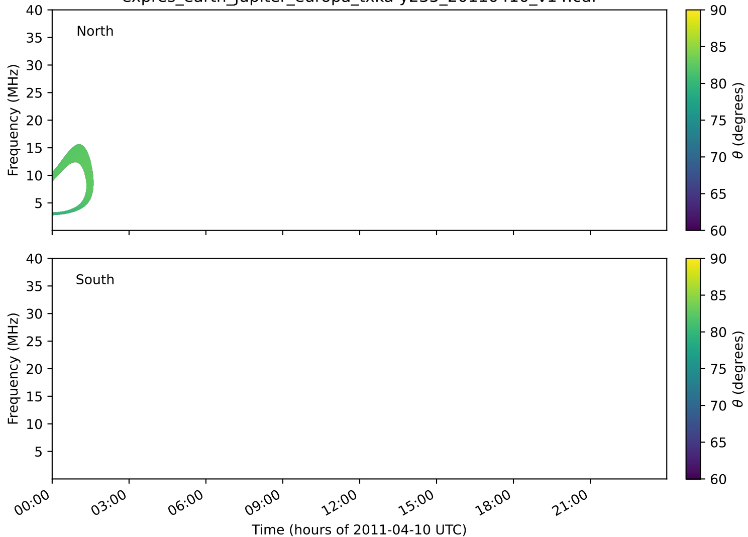
expres_earth_jupiter_europa_txka-y235_20110410_v14.cdf
