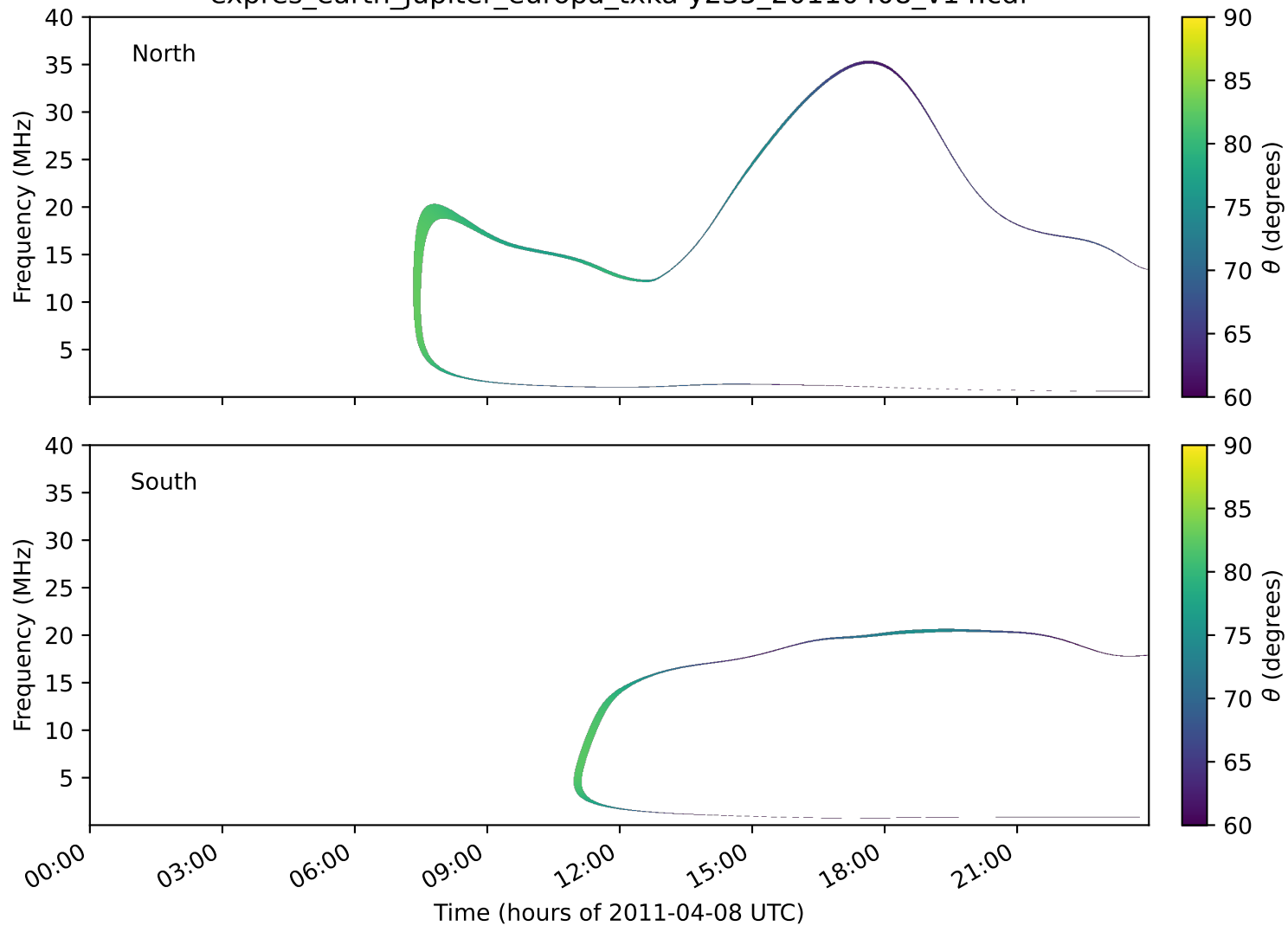
expres_earth_jupiter_europa_txka-y235_20110408_v14.cdf
