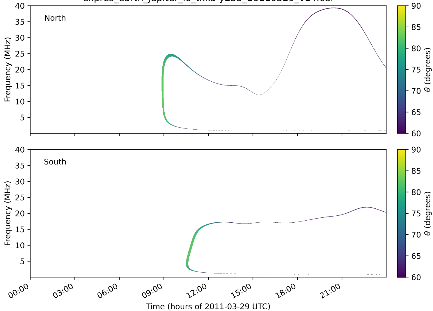
expres_earth_jupiter_io_txka-y235_20110329_v14.cdf
