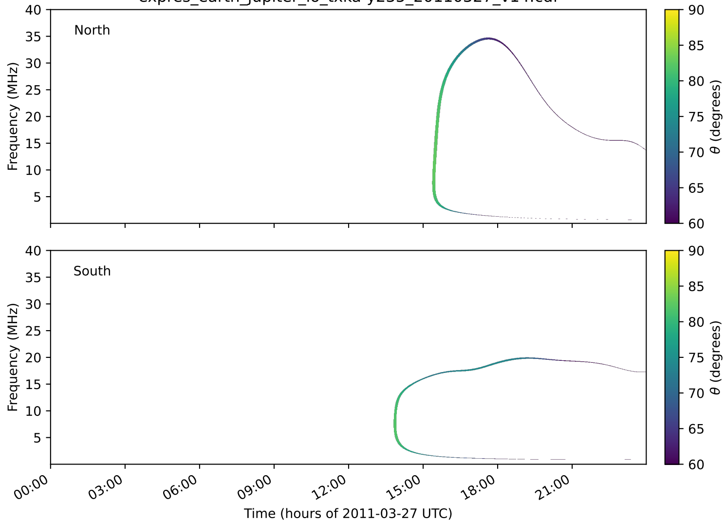
expres_earth_jupiter_io_txka-y235_20110327_v14.cdf
