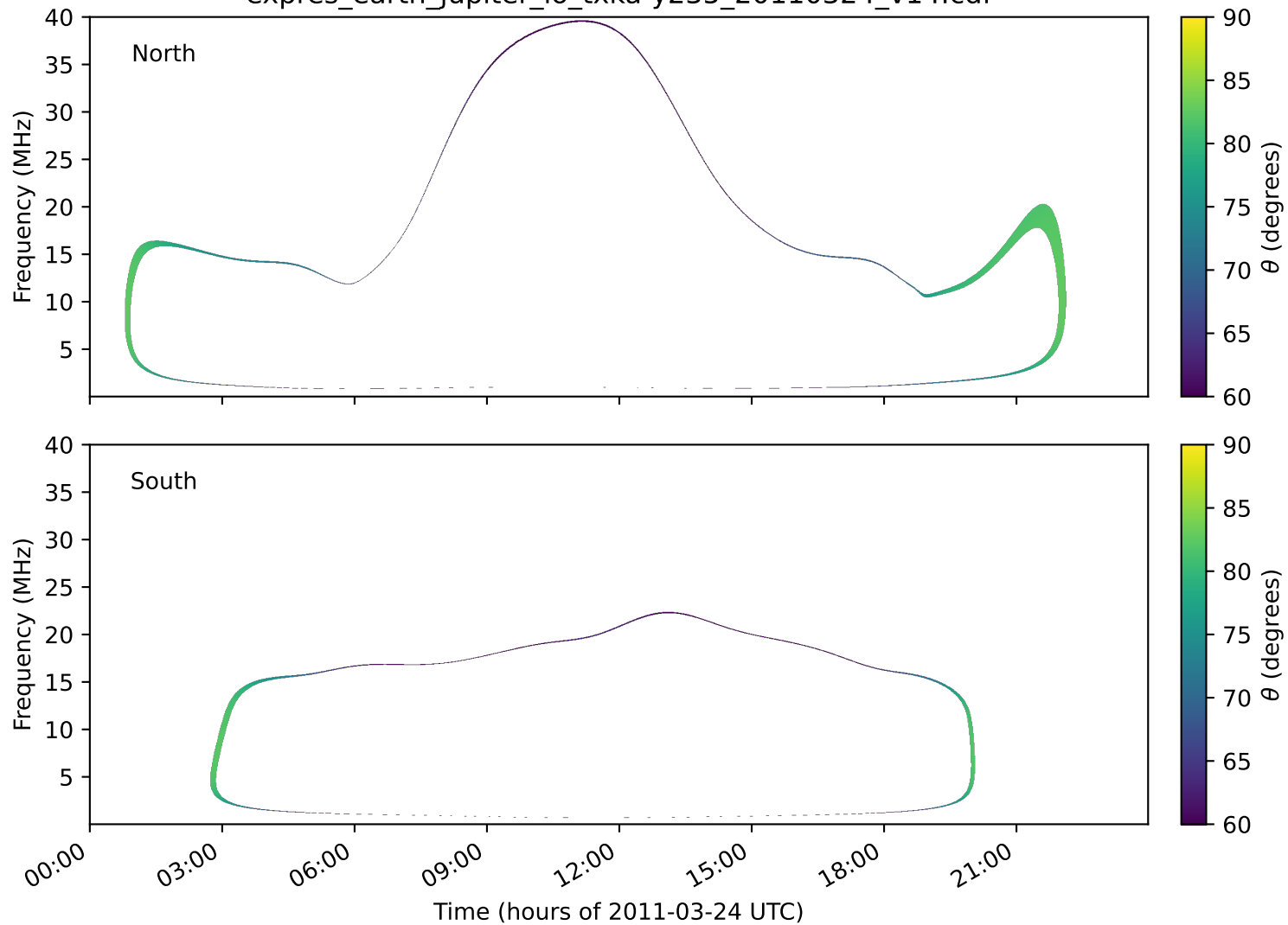
expres_earth_jupiter_io_txka-y235_20110324_v14.cdf
