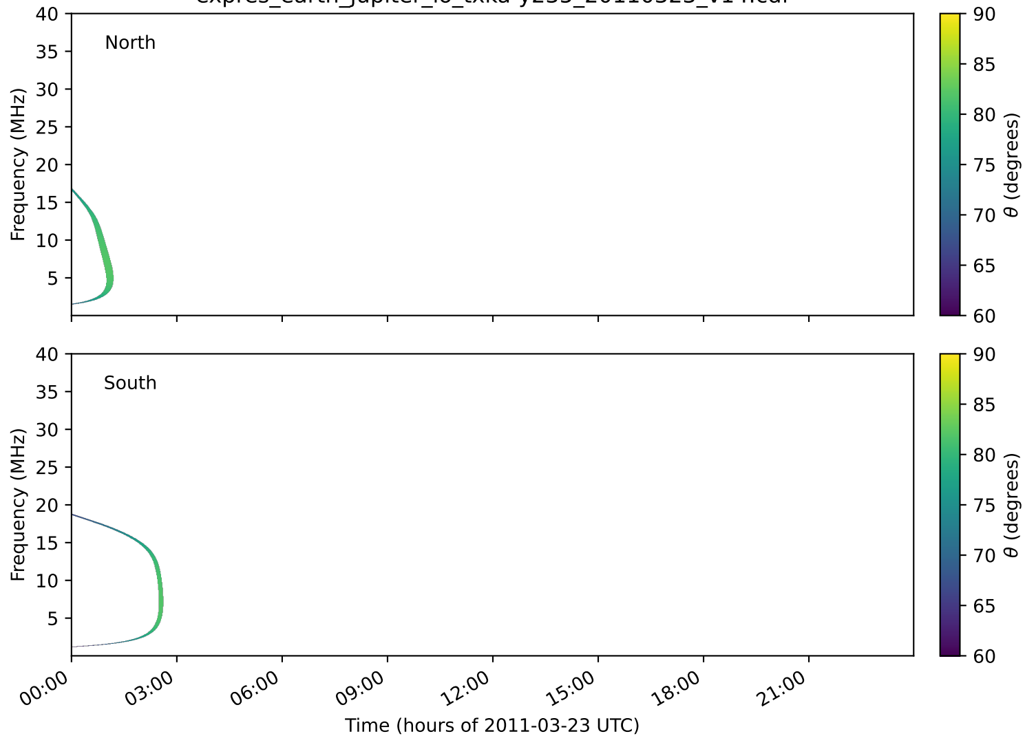
expres_earth_jupiter_io_txka-y235_20110323_v14.cdf
