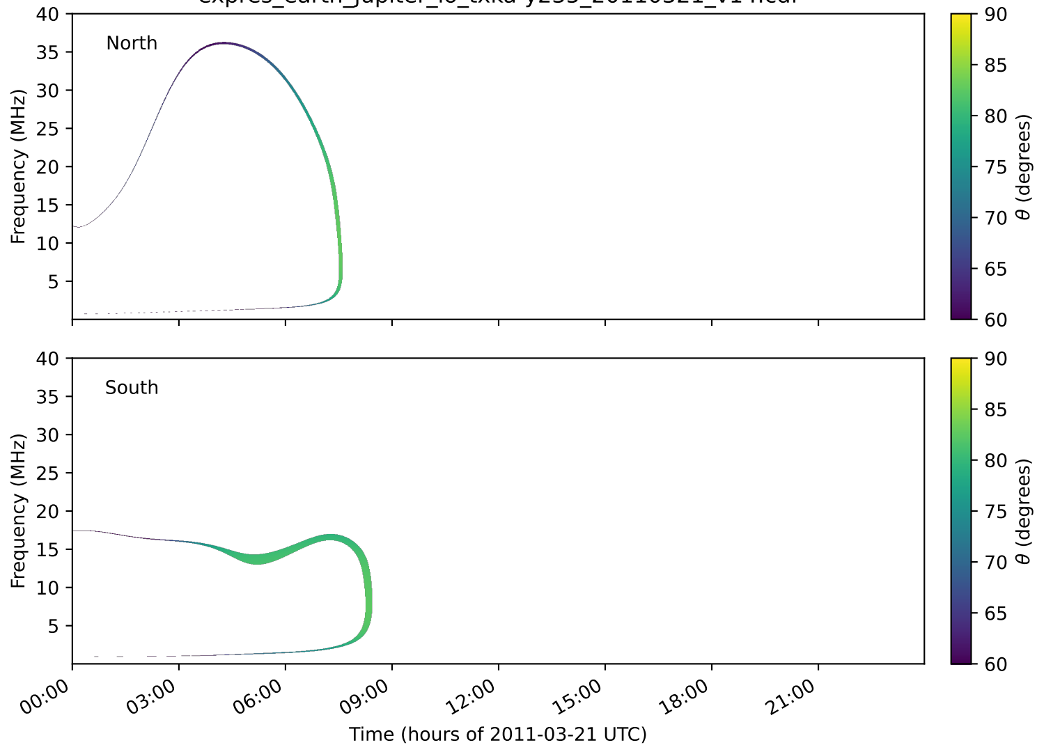
expres_earth_jupiter_io_txka-y235_20110321_v14.cdf
