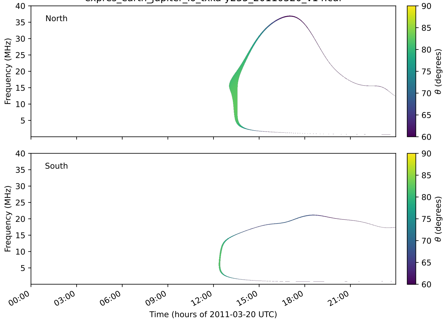
expres_earth_jupiter_io_txka-y235_20110320_v14.cdf
