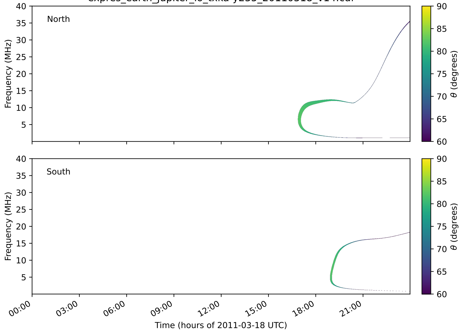
expres_earth_jupiter_io_txka-y235_20110318_v14.cdf
