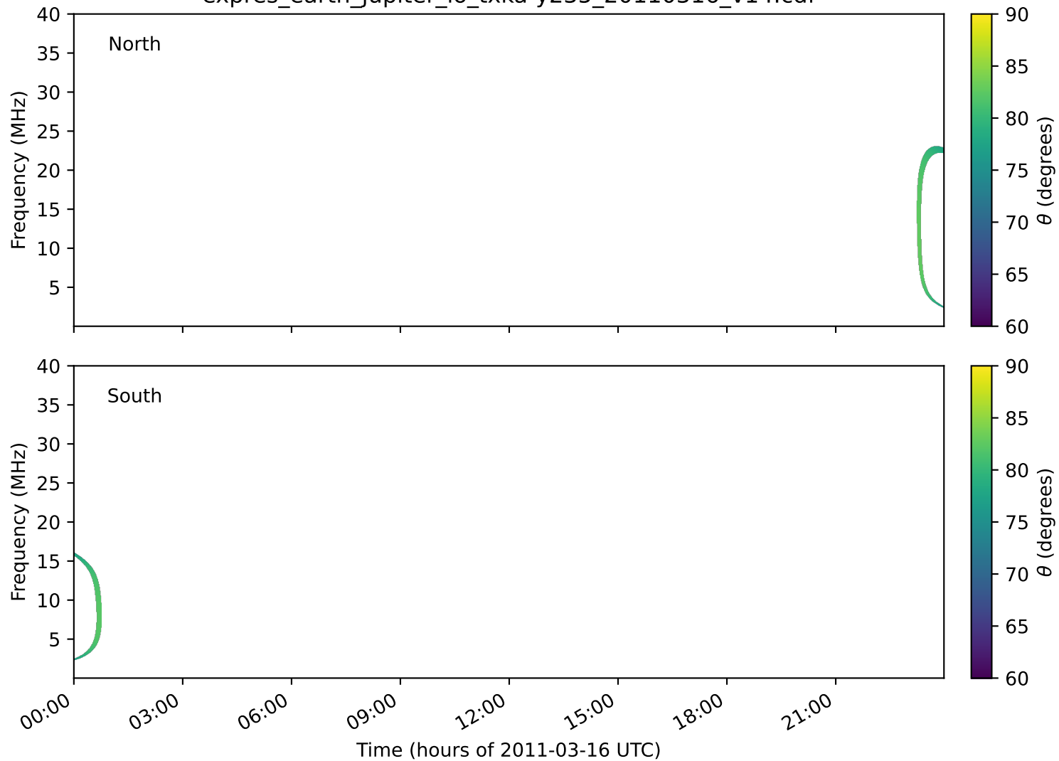
expres_earth_jupiter_io_txka-y235_20110316_v14.cdf
