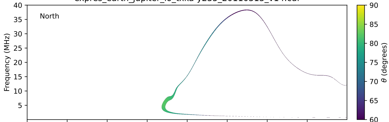
expres_earth_jupiter_io_txka-y235_20110313_v14.cdf
