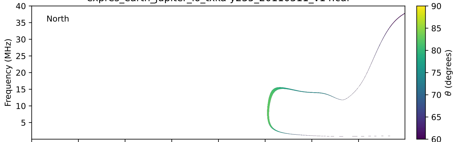
expres_earth_jupiter_io_txka-y235_20110311_v14.cdf
