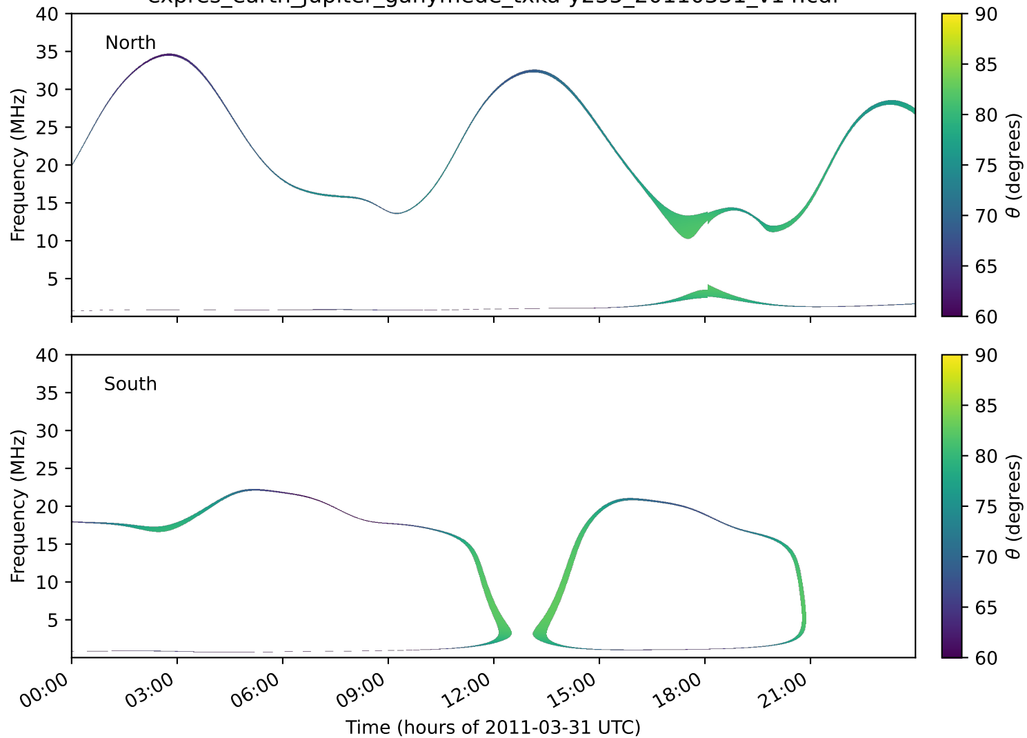
expres_earth_jupiter_ganymede_txka-y235_20110331_v14.cdf
