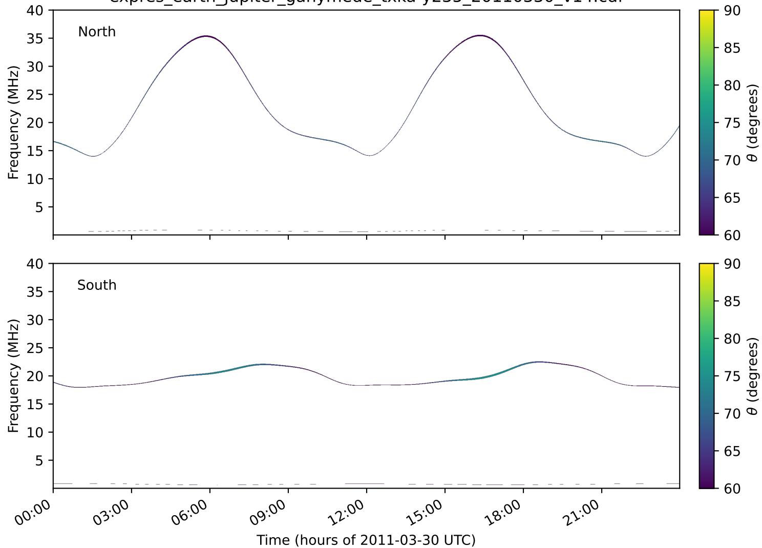
expres_earth_jupiter_ganymede_txka-y235_20110330_v14.cdf
