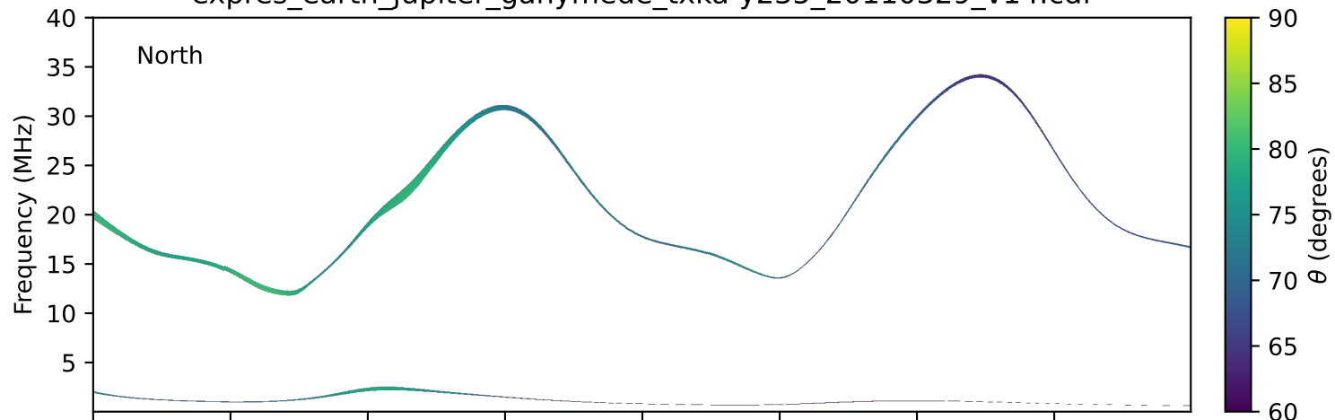
expres_earth_jupiter_ganymede_txka-y235_20110329_v14.cdf
