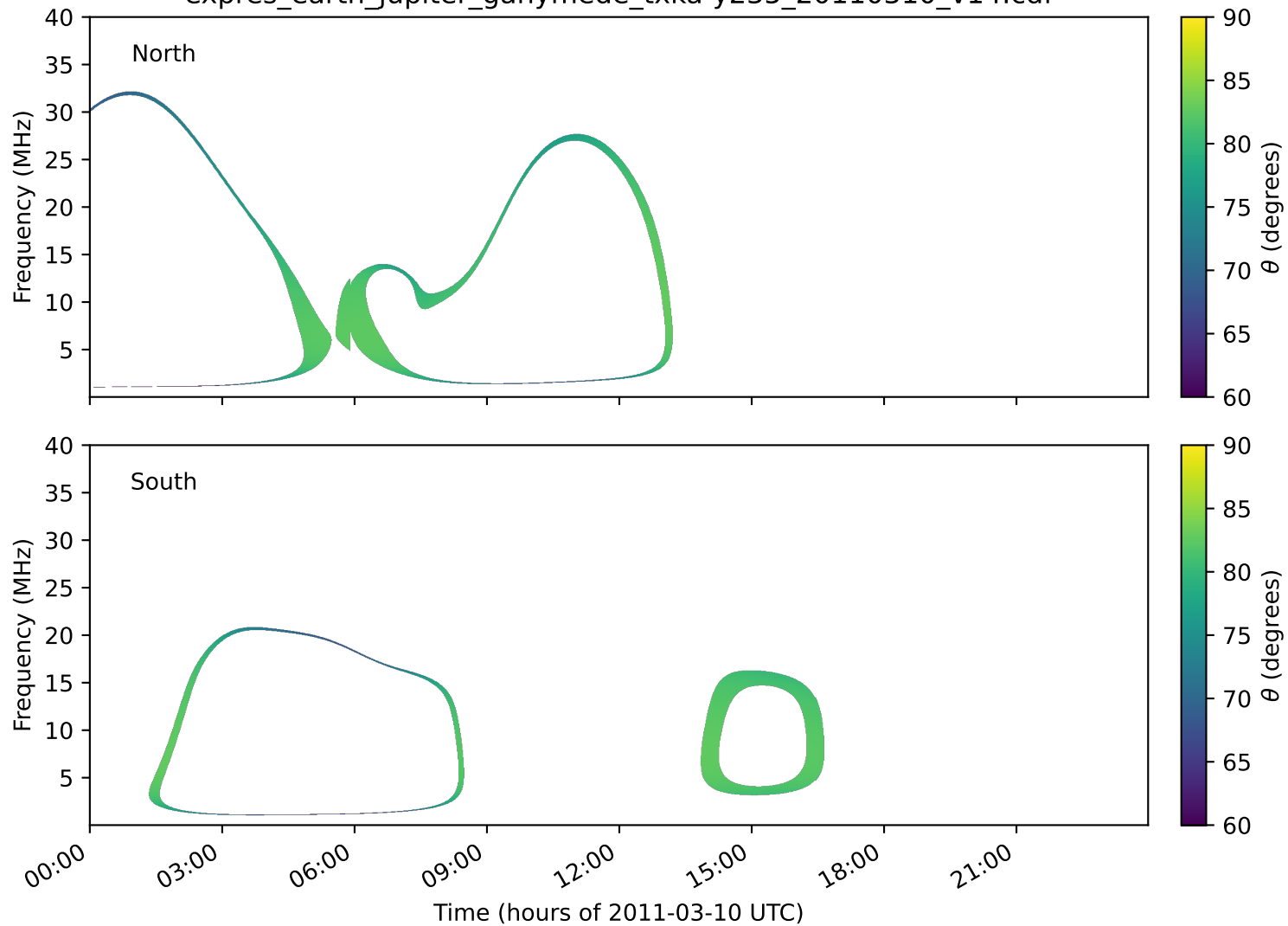
expres_earth_jupiter_ganymede_txka-y235_20110310_v14.cdf
