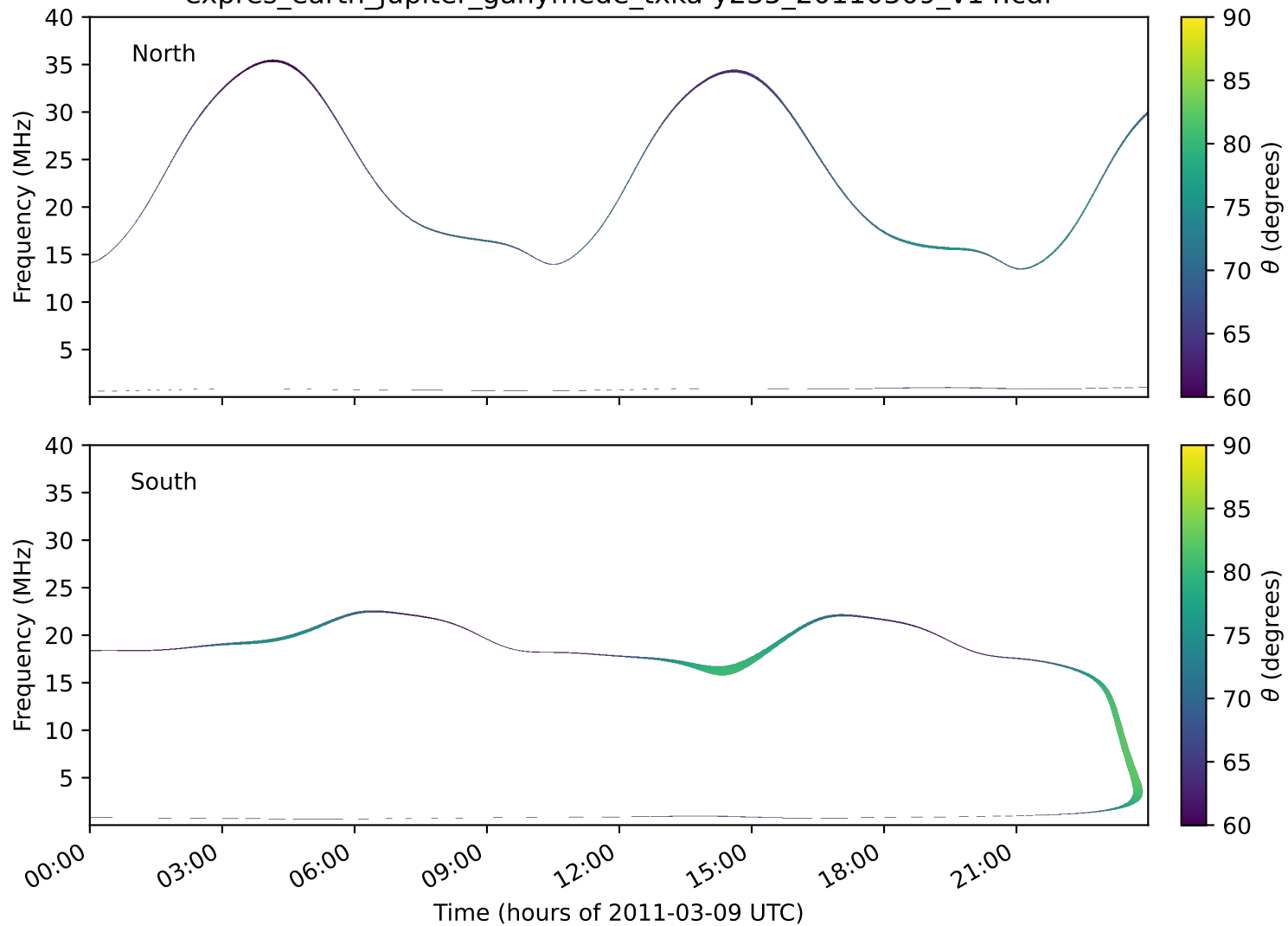
expres_earth_jupiter_ganymede_txka-y235_20110309_v14.cdf
