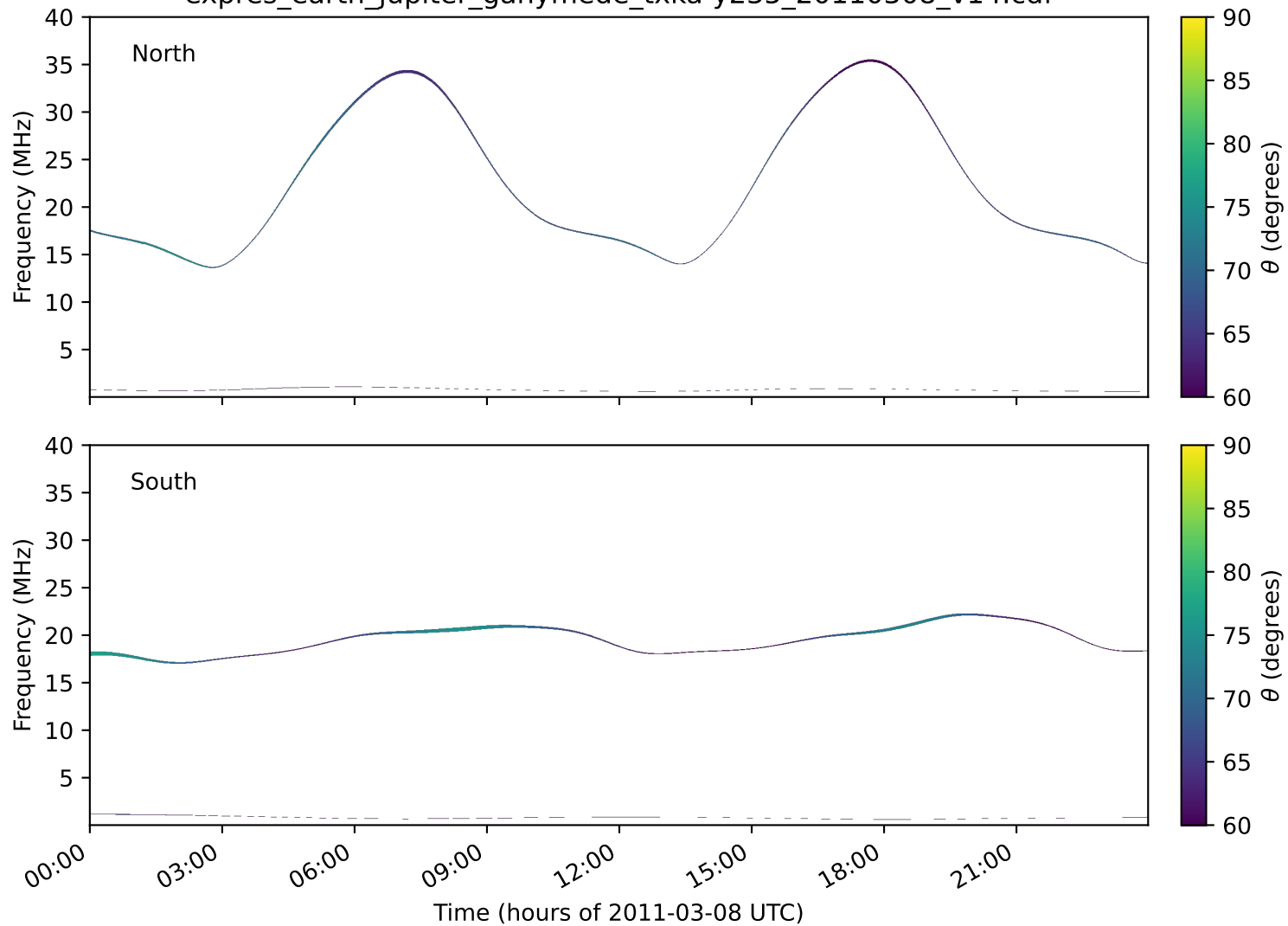
expres_earth_jupiter_ganymede_txka-y235_20110308_v14.cdf
