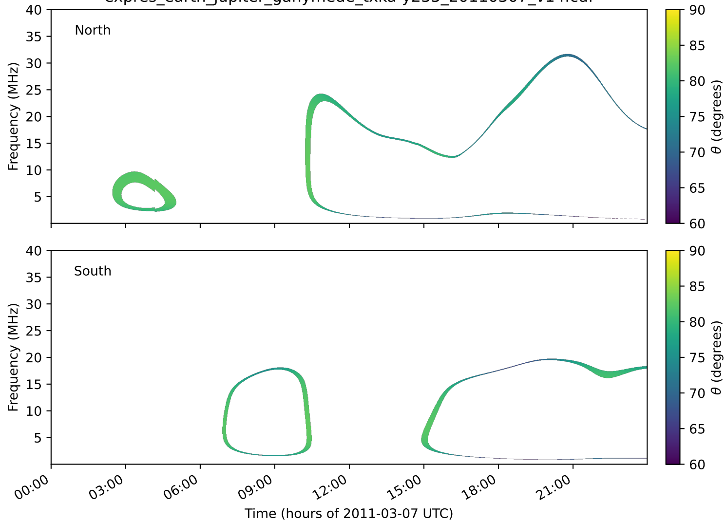
expres_earth_jupiter_ganymede_txka-y235_20110307_v14.cdf
