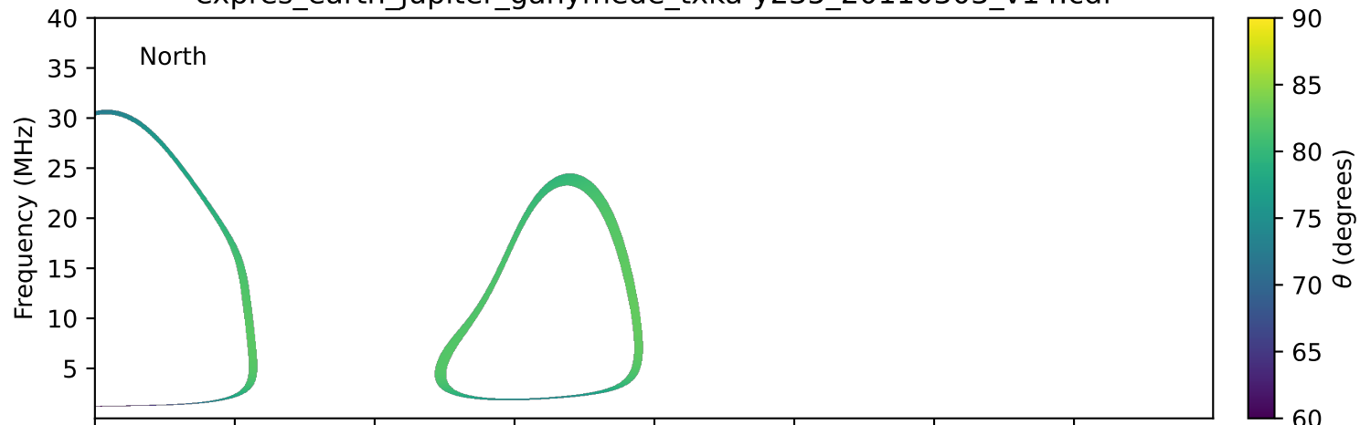
expres_earth_jupiter_ganymede_txka-y235_20110303_v14.cdf
