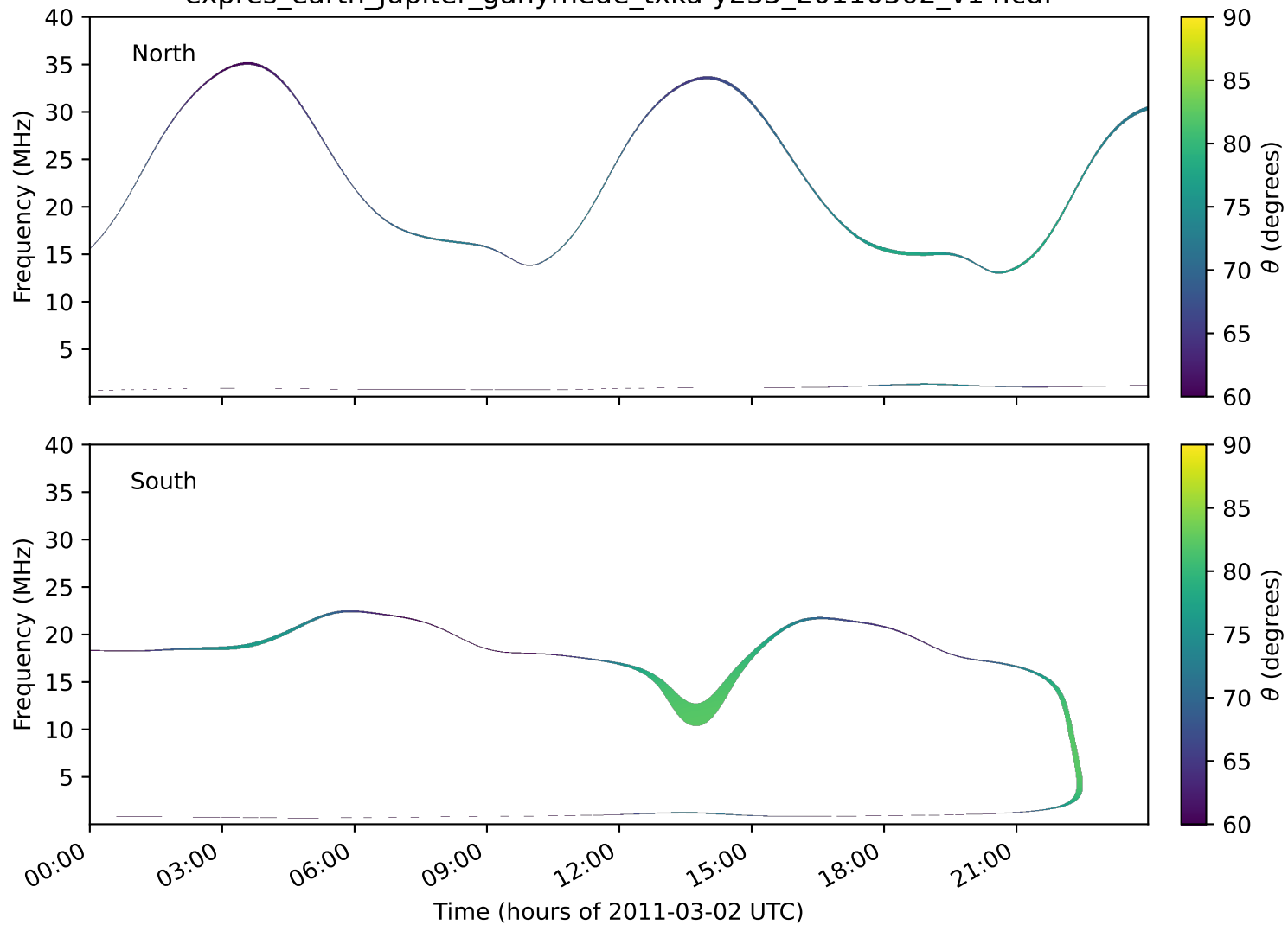
expres_earth_jupiter_ganymede_txka-y235_20110302_v14.cdf
