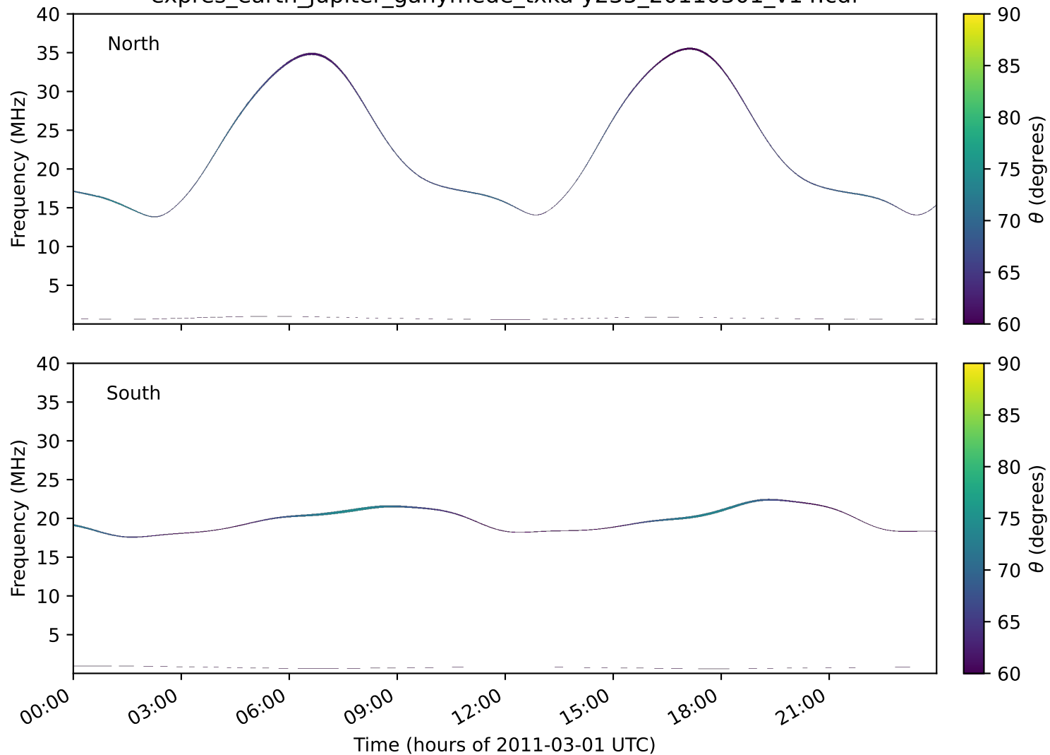
expres_earth_jupiter_ganymede_txka-y235_20110301_v14.cdf
