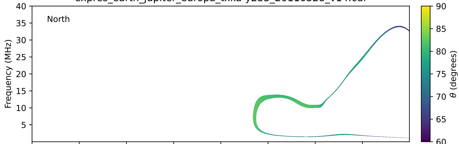
expres_earth_jupiter_europa_txka-y235_20110328_v14.cdf
