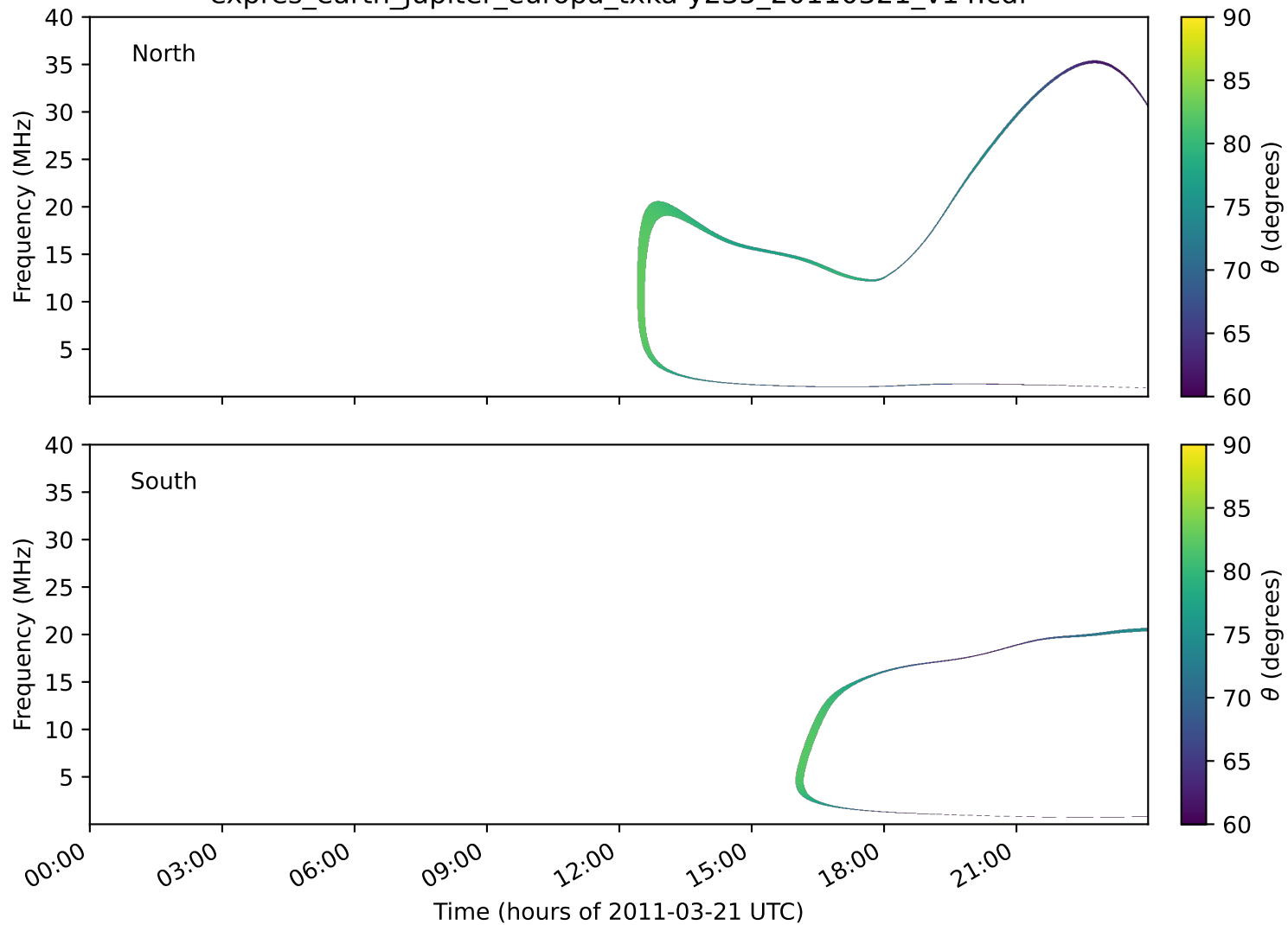
expres_earth_jupiter_europa_txka-y235_20110321_v14.cdf
