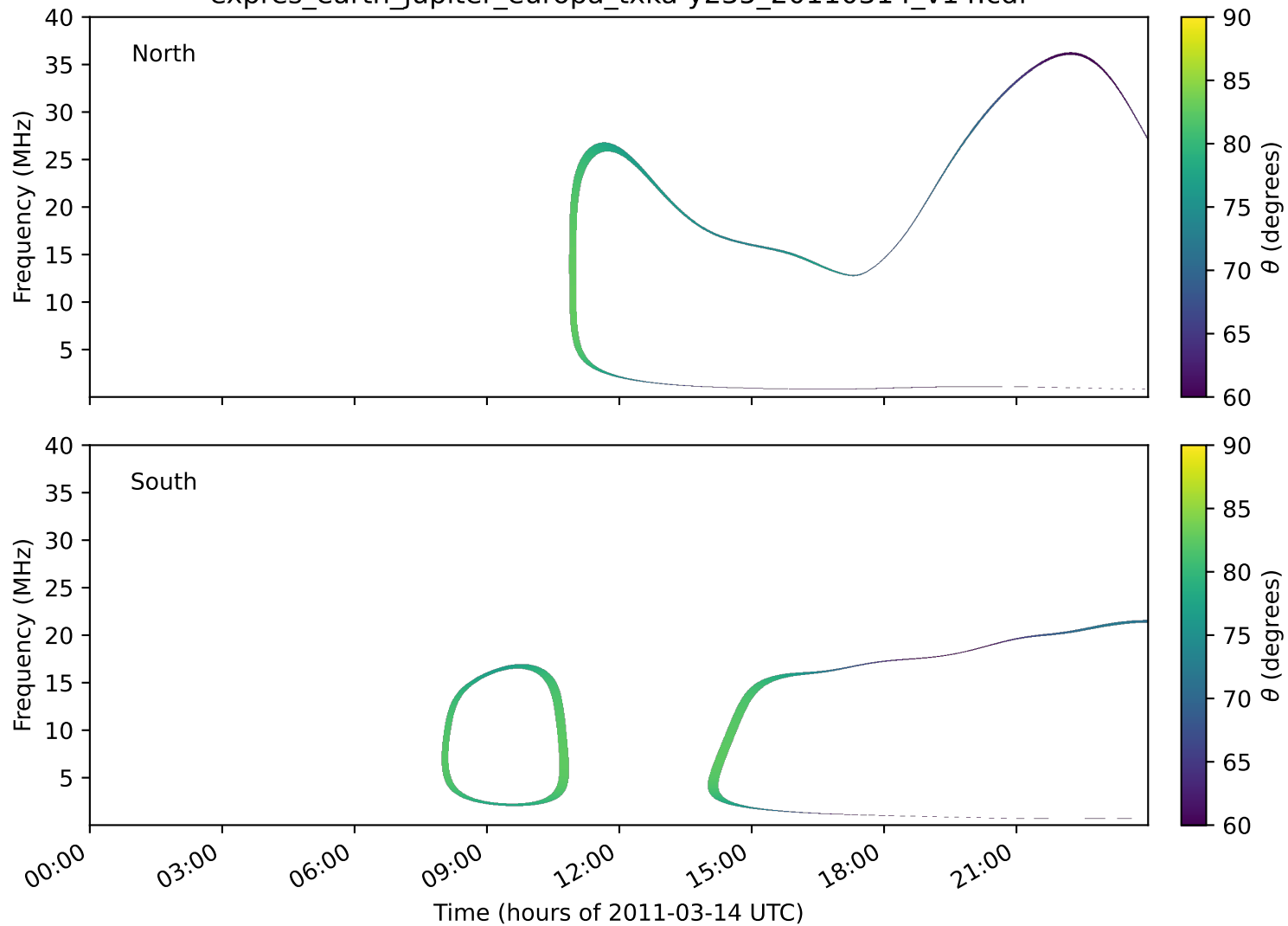
expres_earth_jupiter_europa_txka-y235_20110314_v14.cdf
