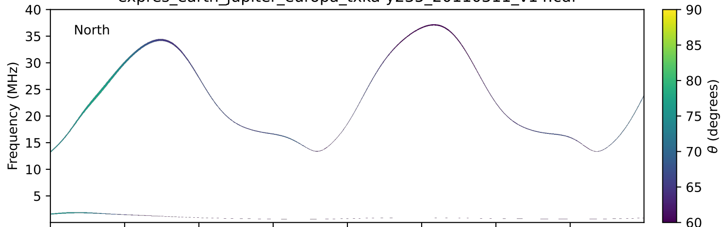
expres_earth_jupiter_europa_txka-y235_20110311_v14.cdf
