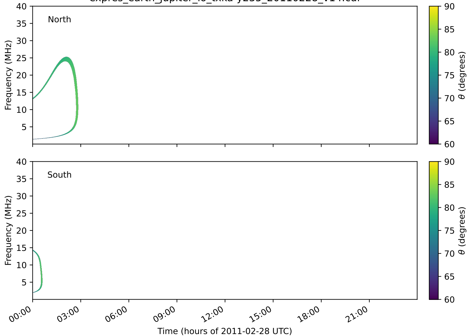
expres_earth_jupiter_io_txka-y235_20110228_v14.cdf
